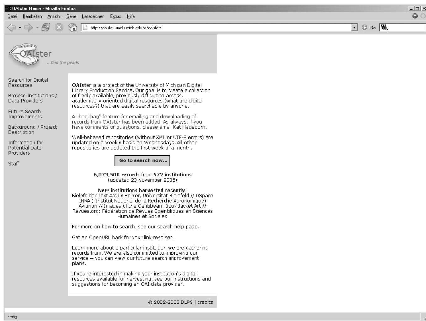
Figure 6. Searching OAIster for 'open access repositories'
